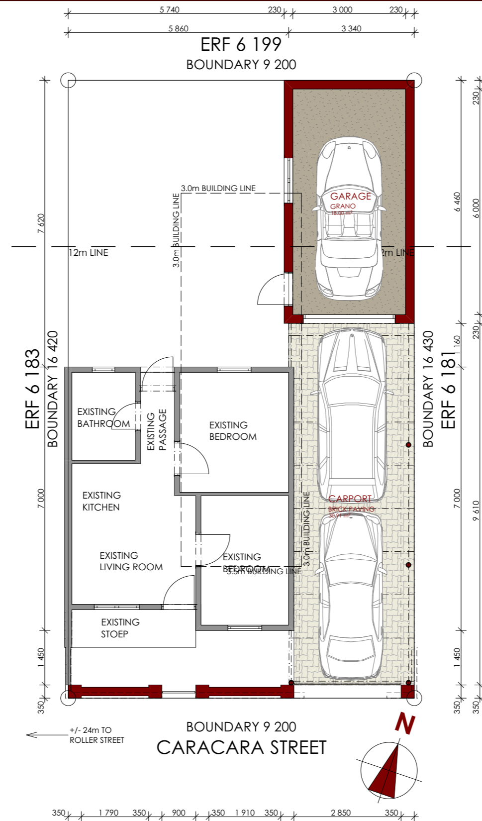
SITE & GROUND FLOOR PLAN
